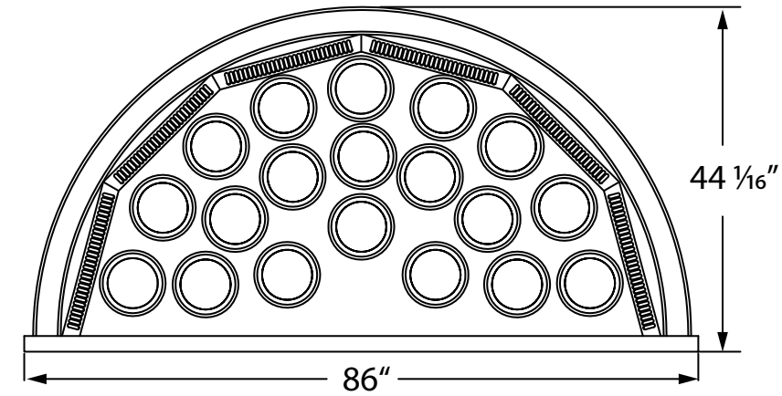
Canopy Removed to Show Total Bucket Count
